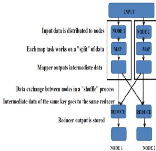
Fig.1.MapReduce Job submission flow mechanism
