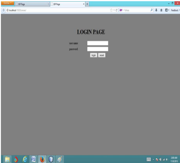
Fig 2: Authentication Step
