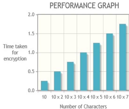
Fig 7: Performance Graph
