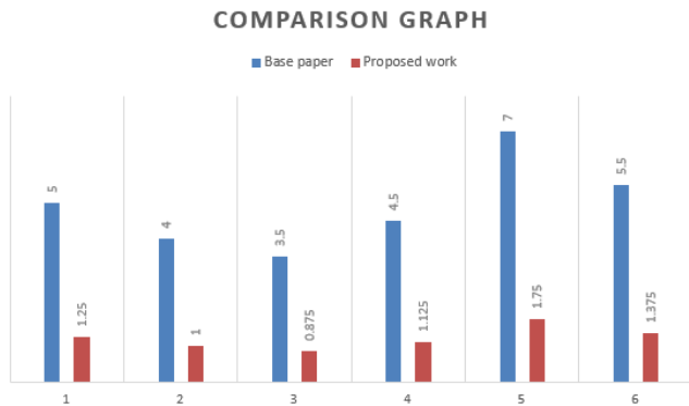
Fig 9: Comparison Evaluation
