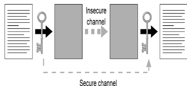
Fig. 1 Example of Conventional Encryption uses a shared key
