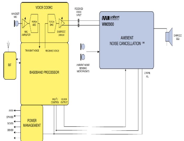
Figure 2 Block diagram of receive active noise cancellation
