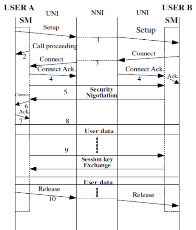
Figure 2: The control flow of ATM connection
