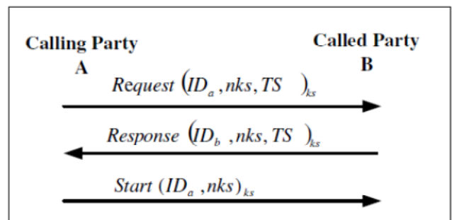
Figure 4: Session key modification protocol
