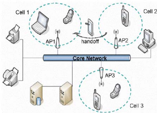
Figure 1: Vertical Handover in heterogeneous networks
