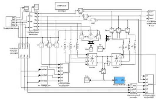
Fig 5: Simulink model of upqc with ANN controller
