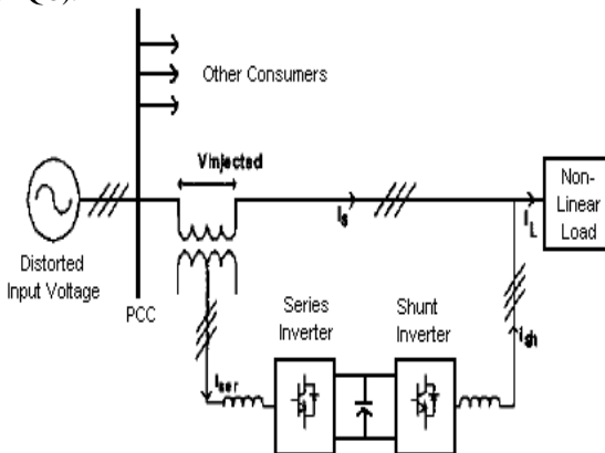
Fig1: Unified Power Quality Conditioner
