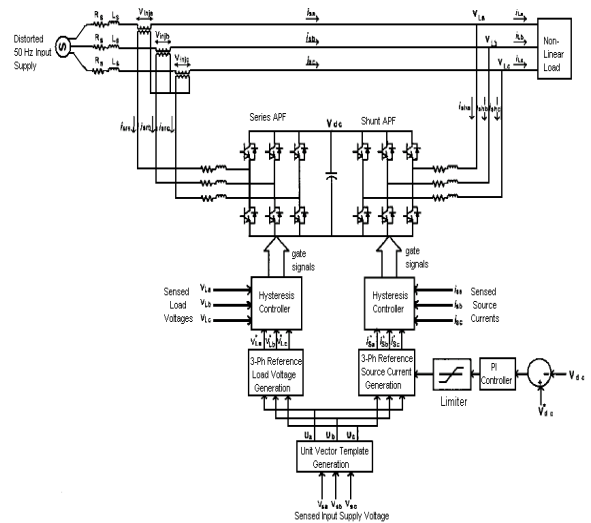
Fig2: Block diagram of UPQC
