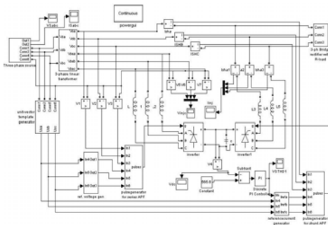
Fig3: Simulink model of upqc with PI controller
